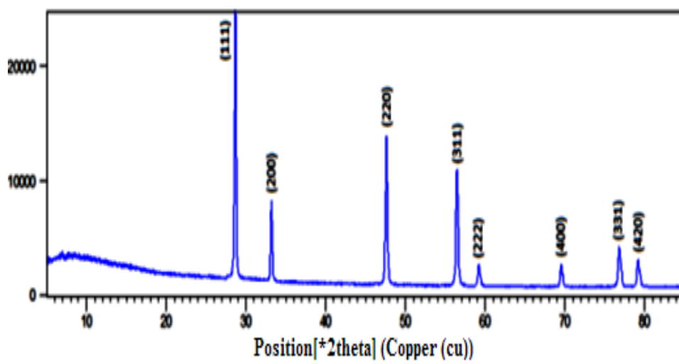
Figure 3. XRD spectra of nano CeO 2
