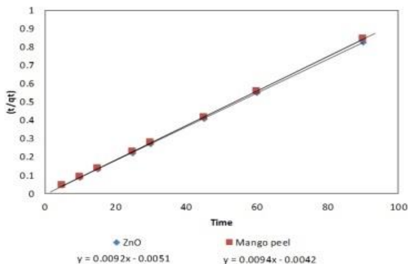
Figure 5. The pseudo-second-order kinetic model for adsorption of blue 221 dye on ZnO and mango peel
