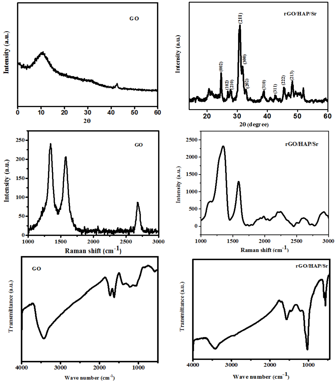
Figure 2. XRD and FT-IR and Raman spectroscopy of GO, and rGO/HAP/Sr nanocomposites
