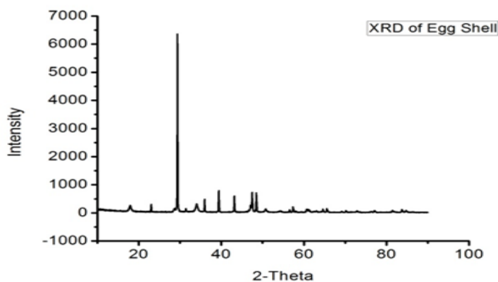
Figure 3. XRD spectra of egg shell (After Calcination)
