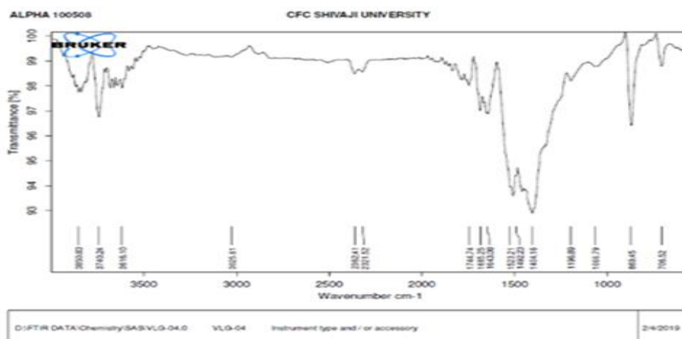
Figure 5. IR spectra of calcinated egg shell
