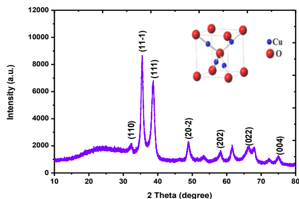
Figure 1. X-ray diffraction profile of synthesized CuO NPs at room temperature
