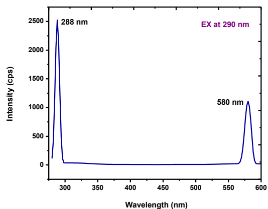
Figure 6. Fluorescence spectra of biosynthesized CuO NPs
