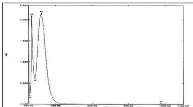
Fig.10. Electronic Spectrum of AuL.
