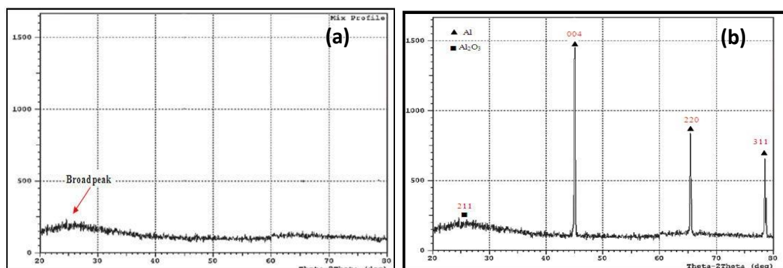
Fig. 4. XRD of AAO template (a) anodized in sulfuric acid, (b) anodized in oxalic acid.
